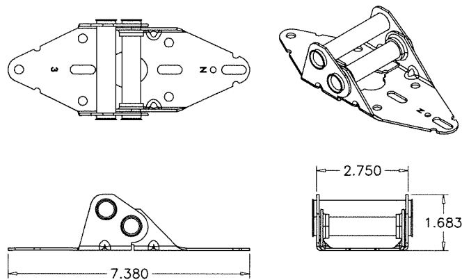
#3 HINGE (11 GA. STEEL)
